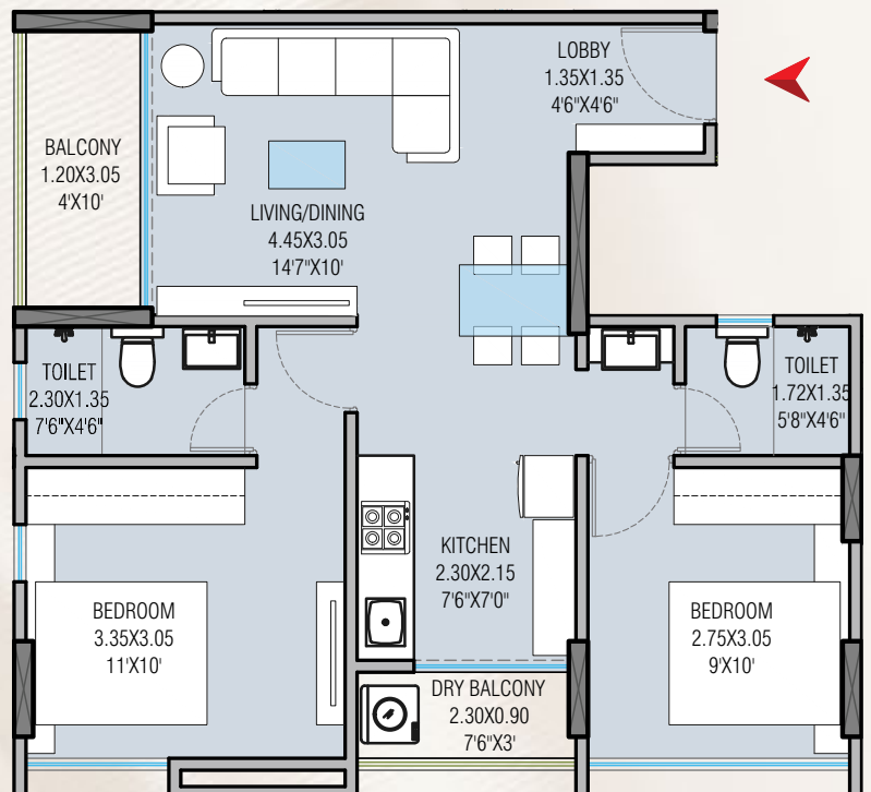
UNIT PLAN | 2BHK - 640 SQ.FT
